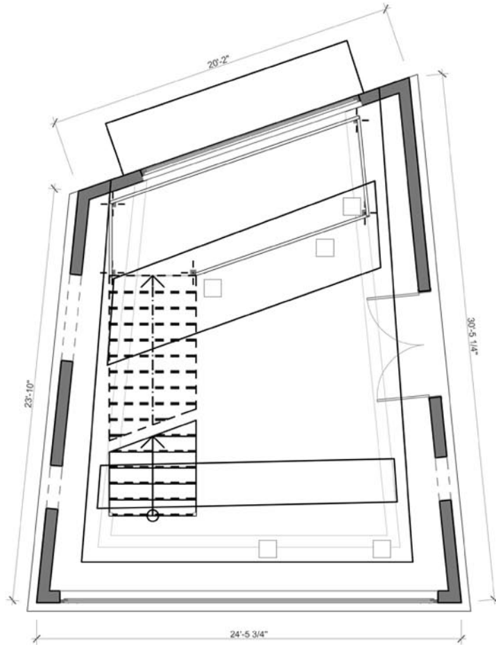
FLOOR PLAN
