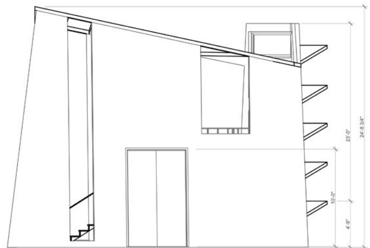
EAST ELEVATION
